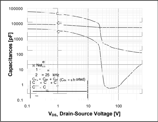
Figure 5. Capacitance Characteristics
